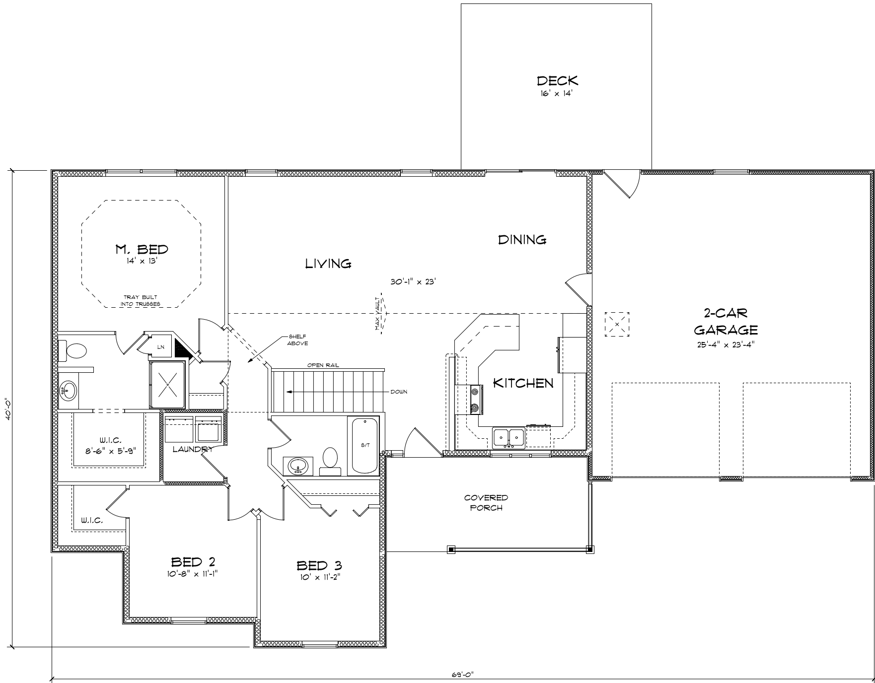
1st FLOOR PLAN 1460 SQ. FT.
